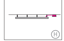
Direct ceiling mounting (white) 50mm / 1.9" with external power supply unit in separate canopy
